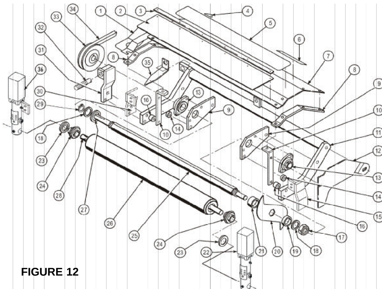
FIGURE 12—VERTICAL MOWING UNIT, Right Hand or Left Hand
