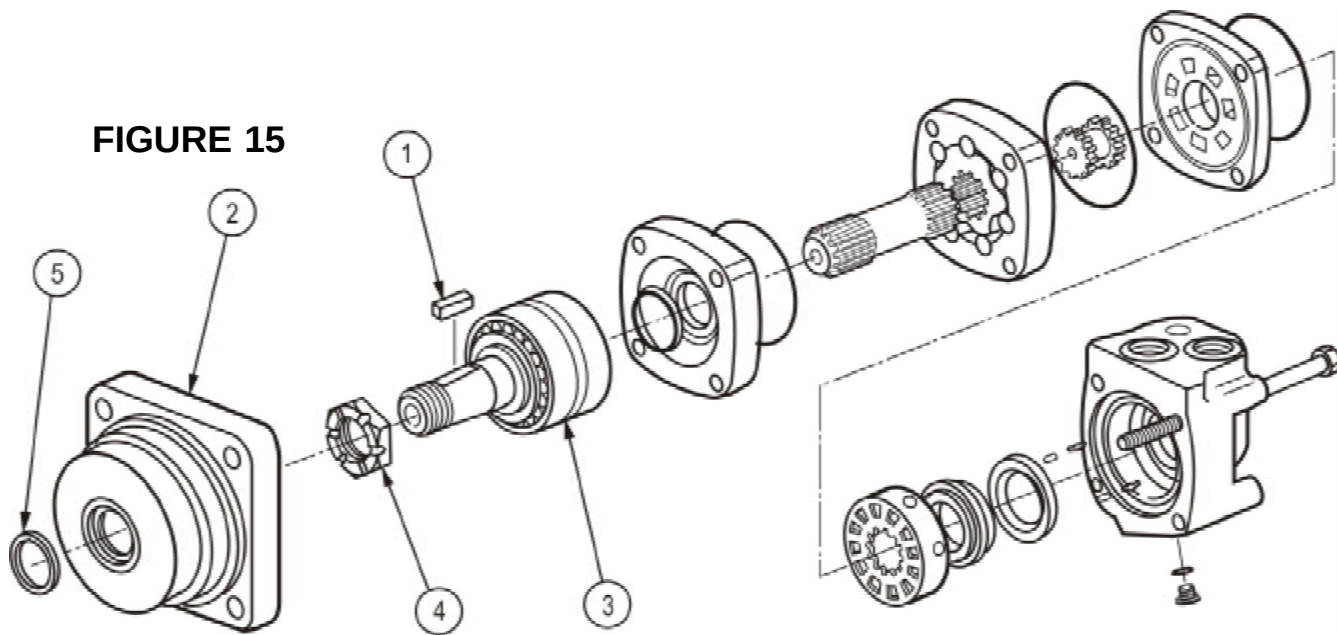
FIGURE 15—WHEEL MOTOR, Part No's. 07273, 07388 & 07390
