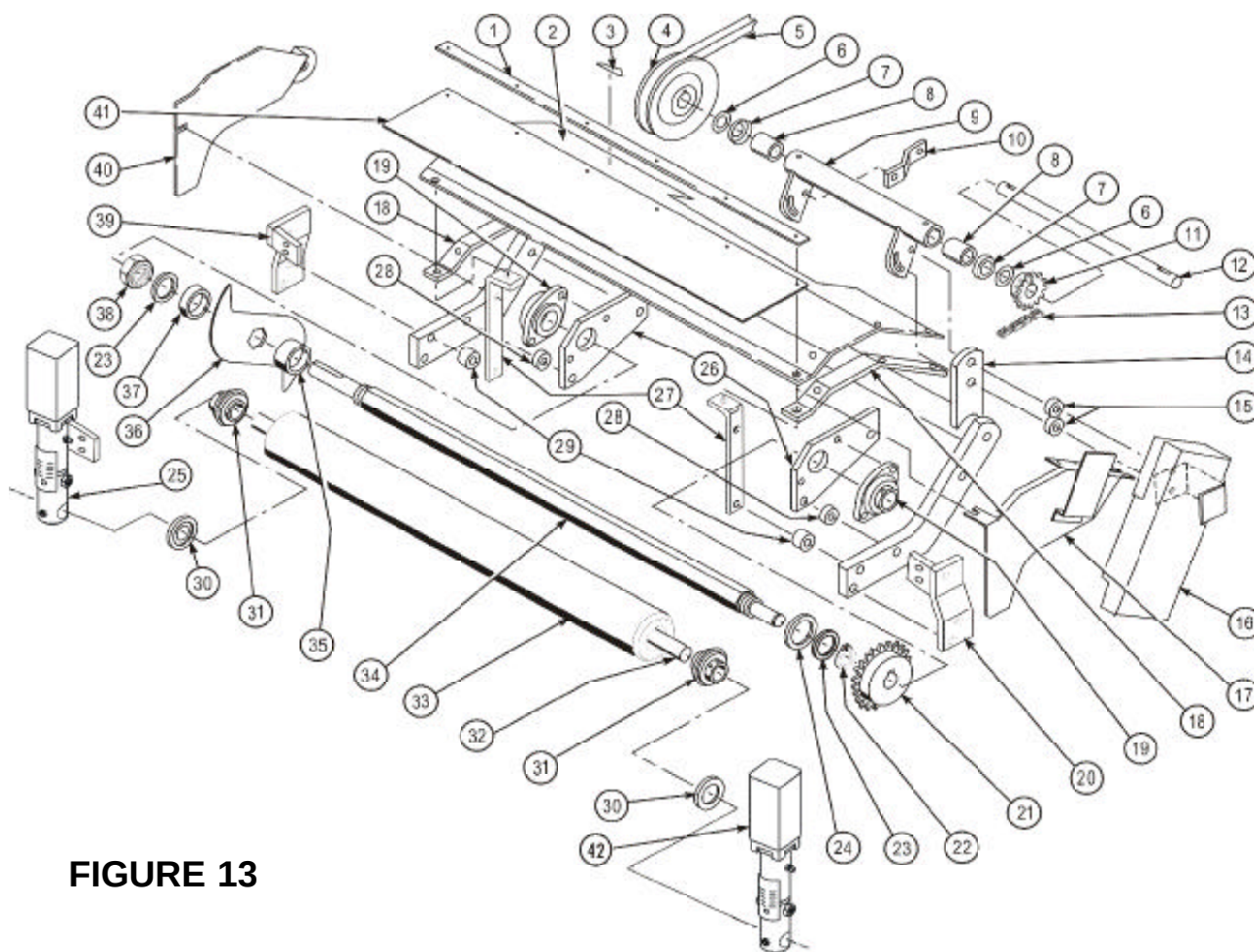
FIGURE 13—VERTICAL MOWING UNIT, Rear
