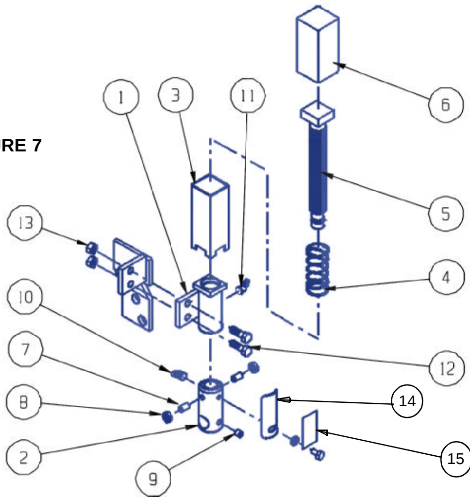
FIGURE 7 — DIAL-A-HEIGHT™ ASSEMBLY
