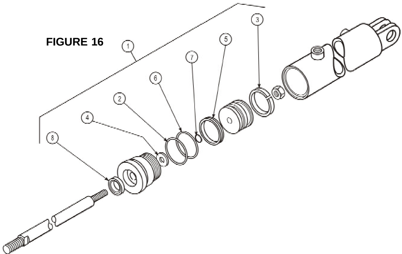
FIGURE 16—STEERING CYLINDER, 204382
