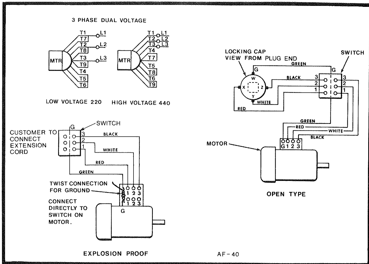
Wiring Diagram
