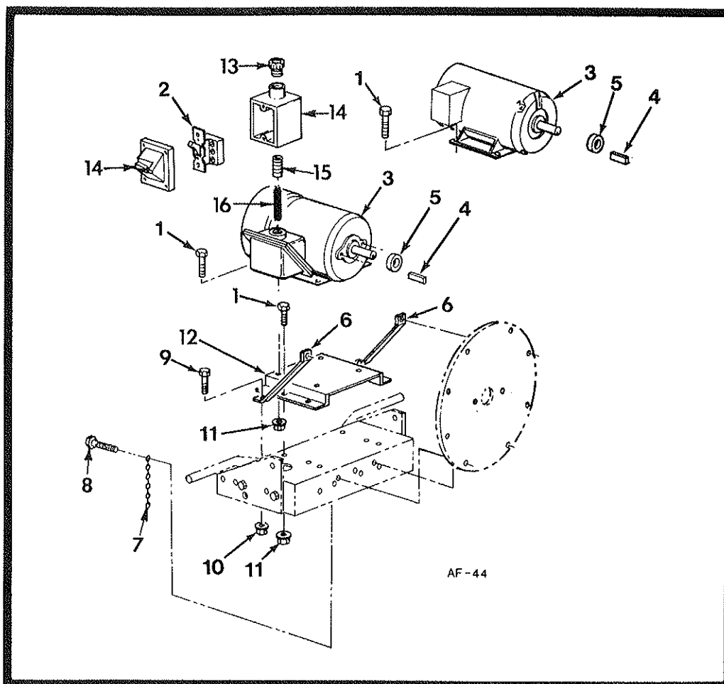
Motor Group
